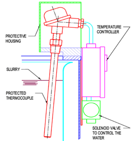
Water Cooling Control Module D-19057
