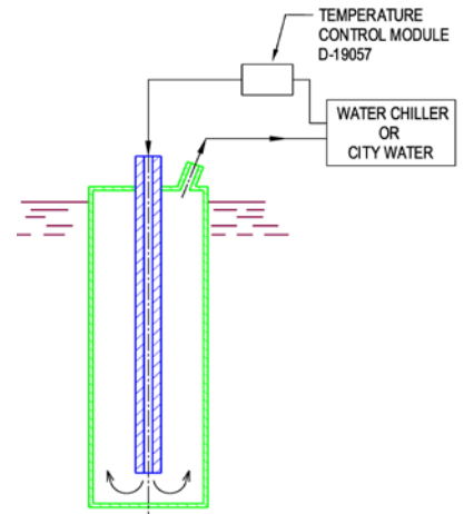
Water Cooling Automatically Controlled
