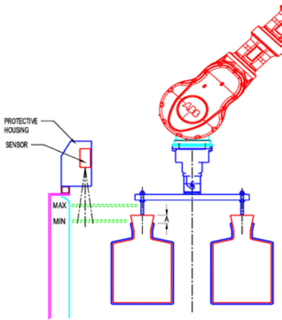
Automatic Slurry Level Sensing
