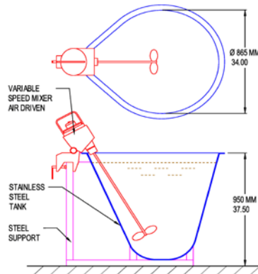
Stationary Premix Tank With Propeller Mixer • Stationary Unit • Mobile Unit
