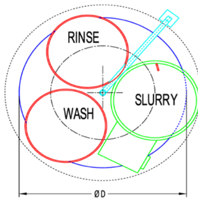
Turntable, Powered Size 1 - 90" Size 2 - 100"
