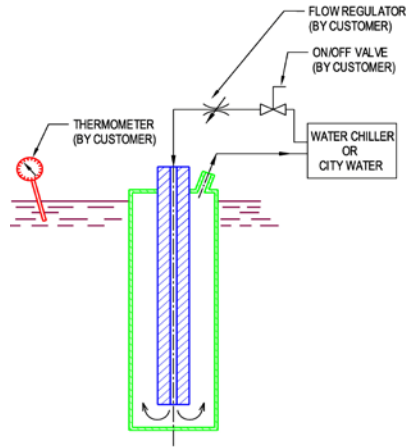
Water Cooling Manually Controlled
