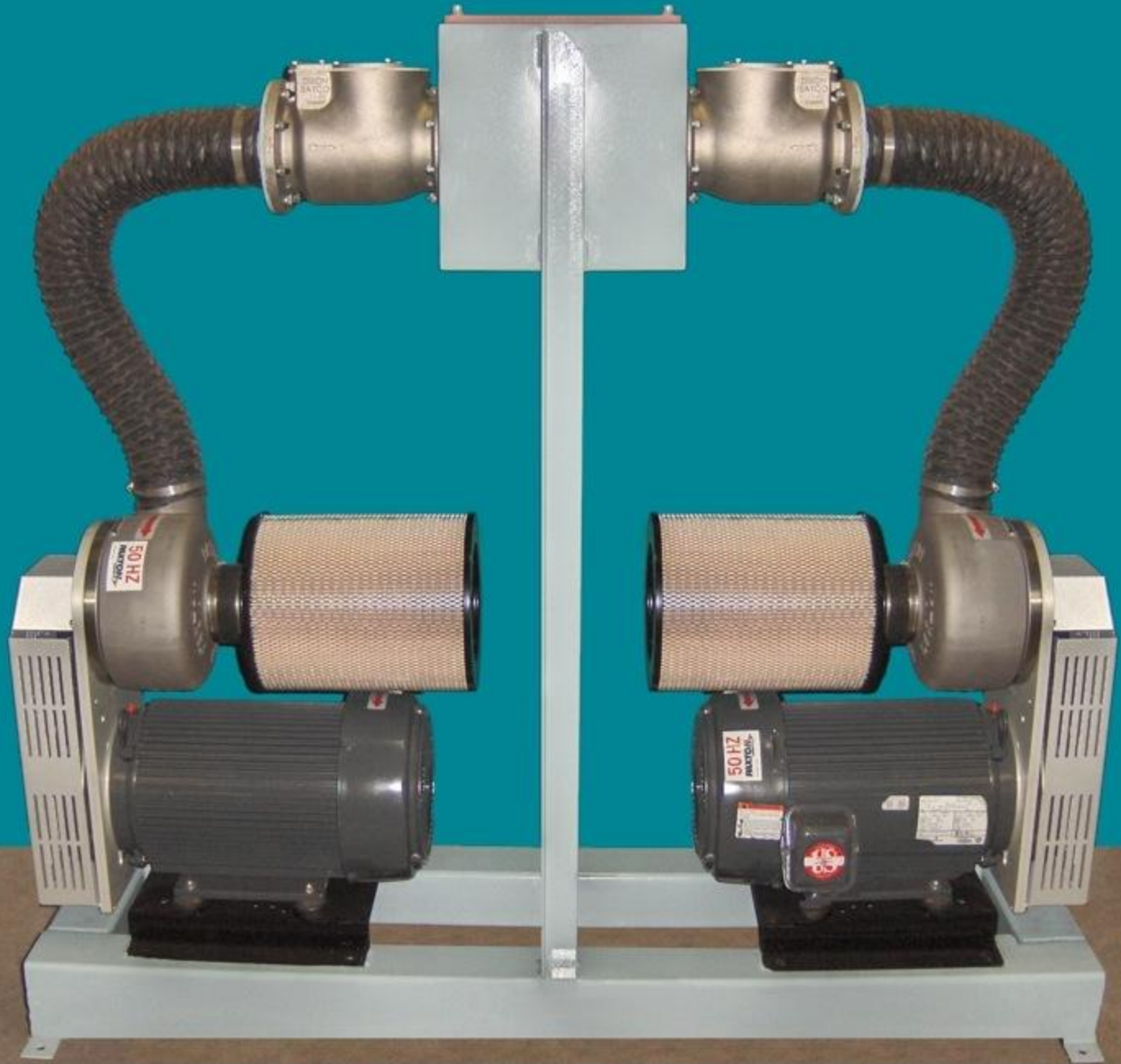
Dual Blower
